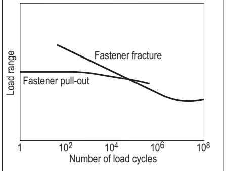
Effect of number of cycles on failure mode DX fastener in steel (incorrectly placed)
