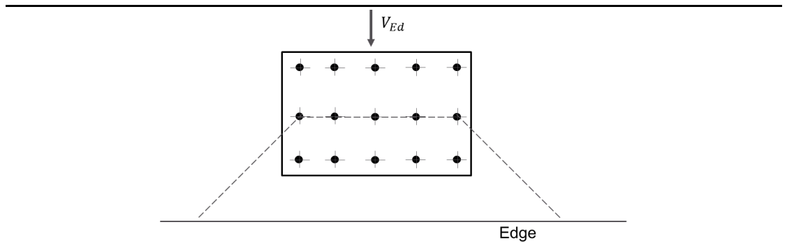
Fig. 4.2: Edge break-out for anchors 5x3 layout close to edge and loaded in shear for static and seismic
