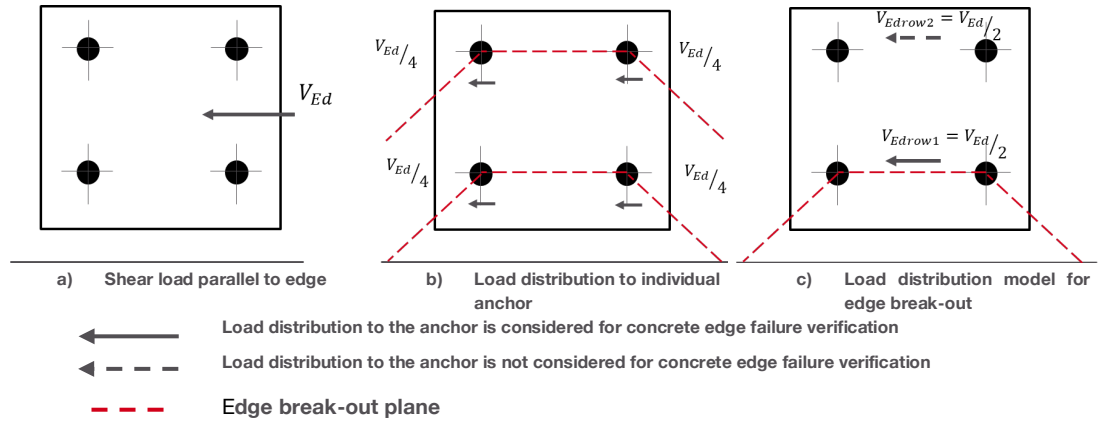
Fig. 4.6: Parallel shear distribution and edge break-out model as per SOFA
