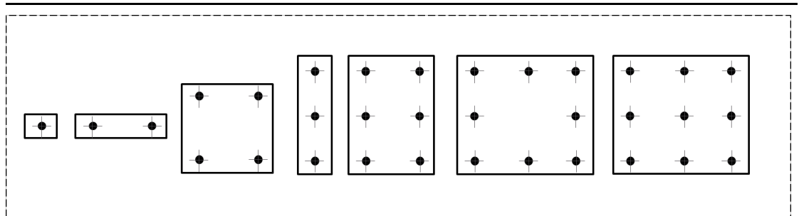
Fig. 2.1: Anchor groups without hole clearance for all edge distances covered by EN 1992-4
