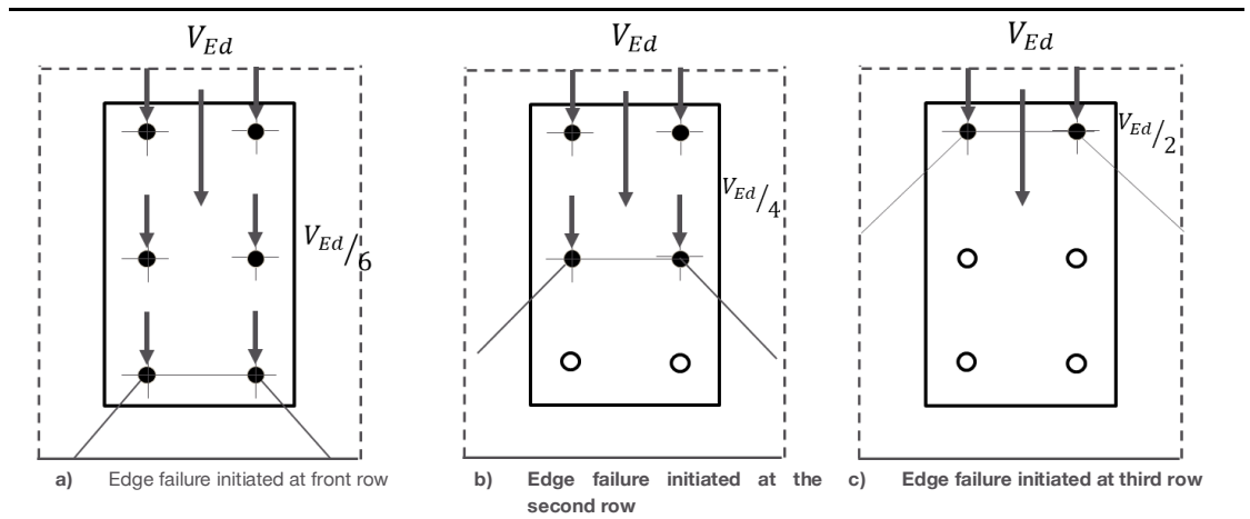
Fig. 3.1: Perpendicular shear load distribution and edge failure in the scope of fib Bulletin 58
